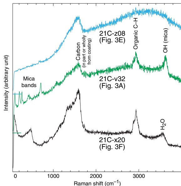
Fig. 4. Raman spectra of glassy matrix of selected grains. Spectra from three grains shown in Fig. 3, with labeled band peaks.
